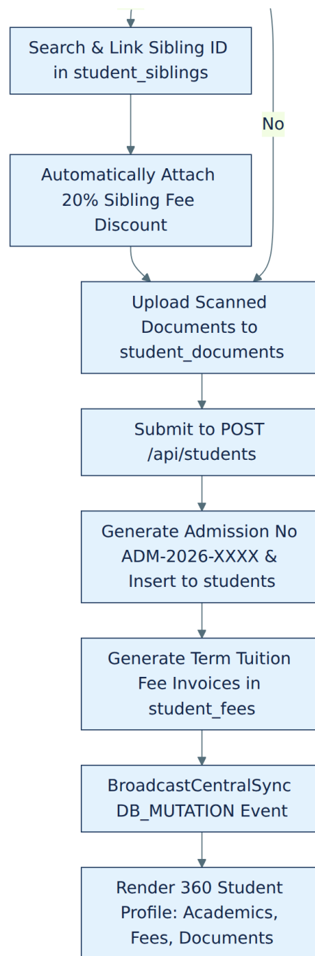
Figure 3: Flowchart 2: Student admission and 360° profile lifecycle (part 2 of 2)
