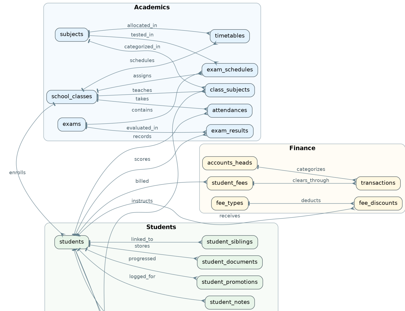
Figure 7: Entity-relationship diagram (56-table schema, key entities) (part 1 of 2)
