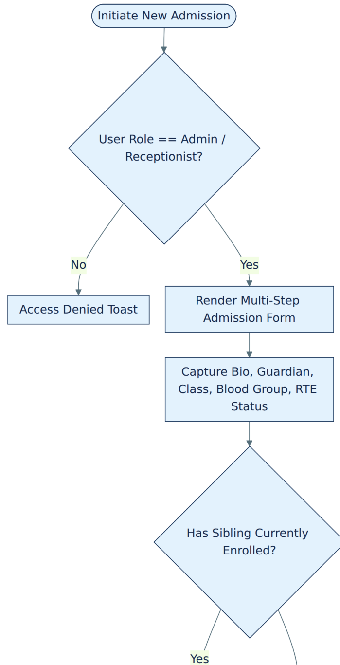
Figure 3: Flowchart 2: Student admission and 360° profile lifecycle (part 1 of 2)
