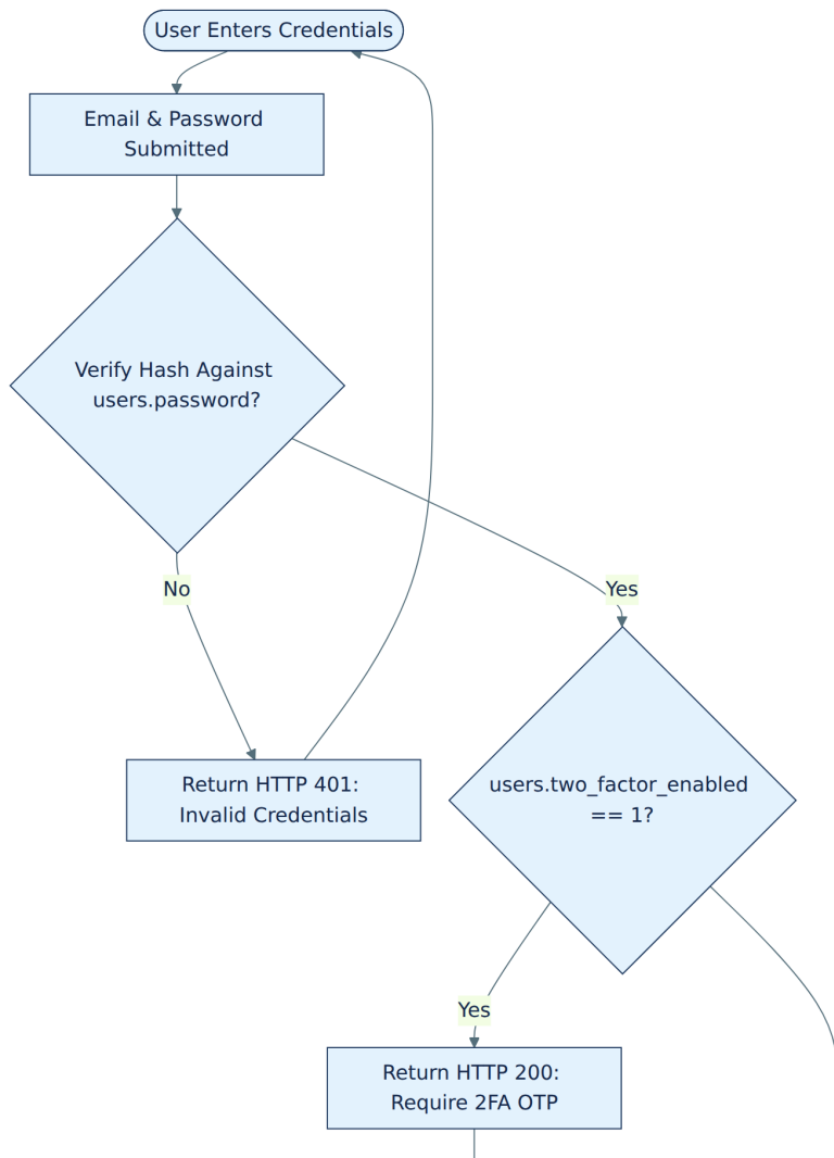
Figure 2: Flowchart 1: Authentication, session and 2FA (part 1 of 2)
