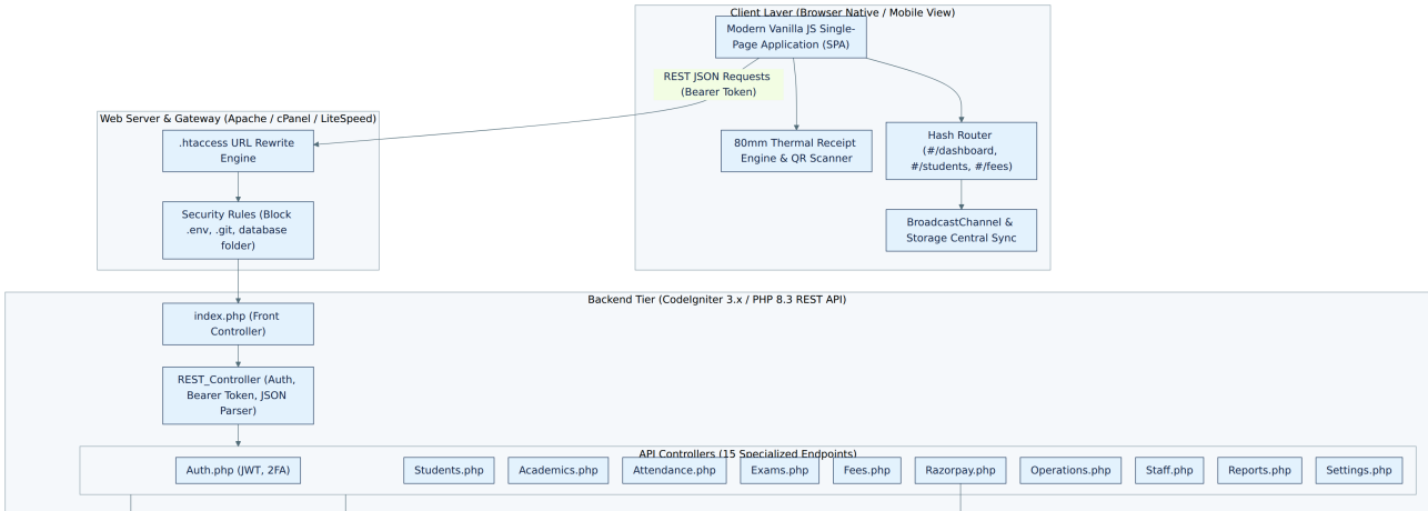
Figure 1: High-level system architecture (part 1 of 2)
