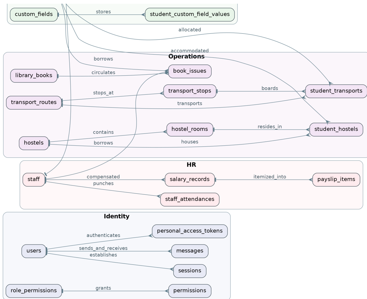
Figure 7: Entity-relationship diagram (56-table schema, key entities) (part 2 of 2)
