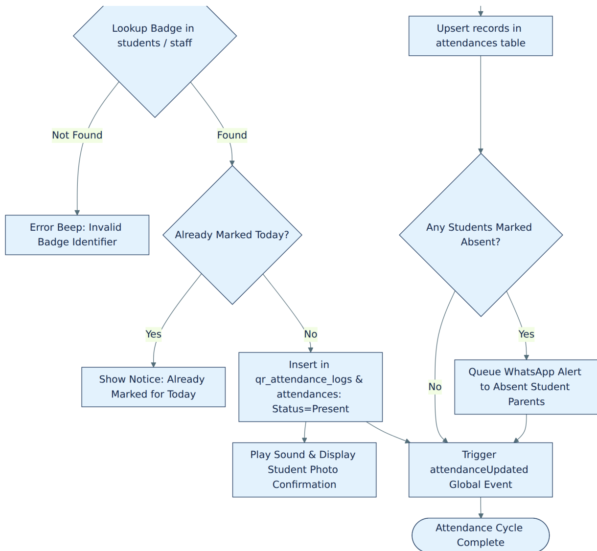
Figure 5: Flowchart 4: Attendance roll call (manual and QR scan) (part 2 of 2)
