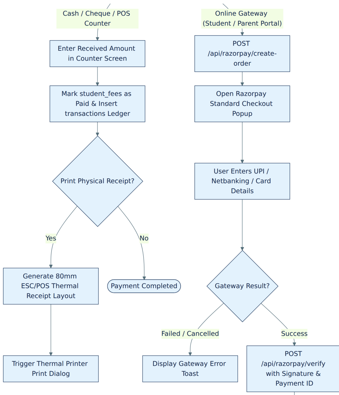
Figure 4: Flowchart 3: Fee billing, fine calculation and Razorpay payment (part 2 of 3)
