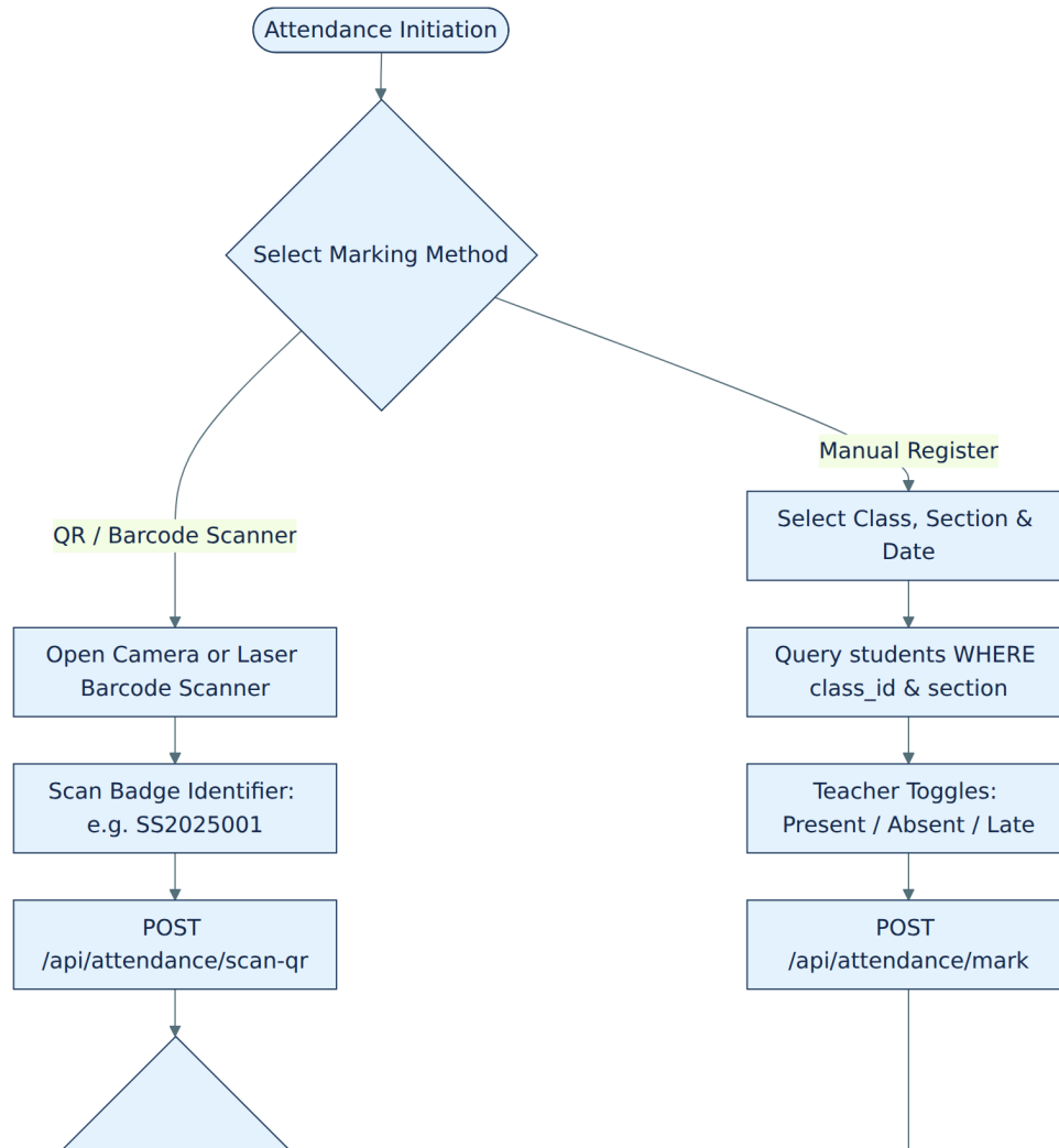
Figure 5: Flowchart 4: Attendance roll call (manual and QR scan) (part 1 of 2)
