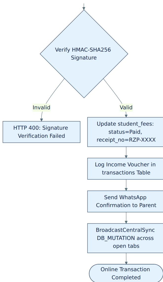
Figure 4: Flowchart 3: Fee billing, fine calculation and Razorpay payment (part 3 of 3)
