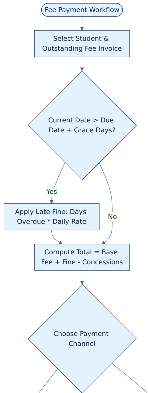
Figure 4: Flowchart 3: Fee billing, fine calculation and Razorpay payment (part 1 of 3)
