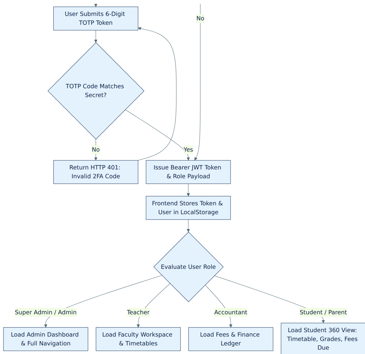
Figure 2: Flowchart 1: Authentication, session and 2FA (part 2 of 2)
